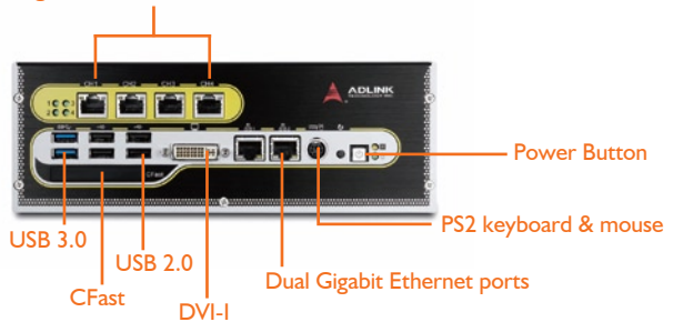
EOS-1200 Front View
